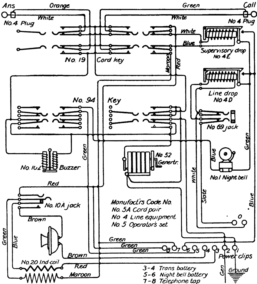
FIG. 99.—Circuits of fifty-drop, North Electric, magneto switchboard.
